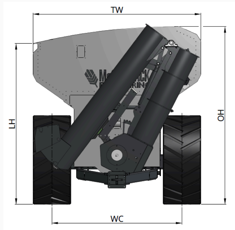
Transport Position
