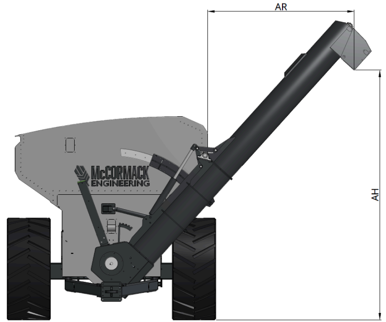
Auger Halfway
