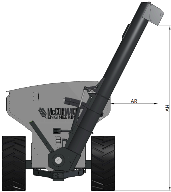
Auger Up
